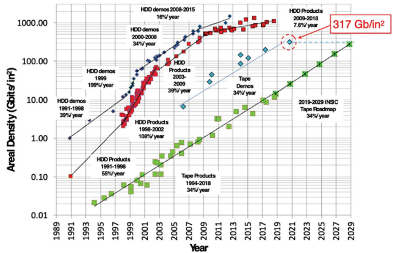
317 Gb/in 2 demonstrates the sustainability of the INSC Tape Roadmap 34% CAGR in Areal Density for the next decade
